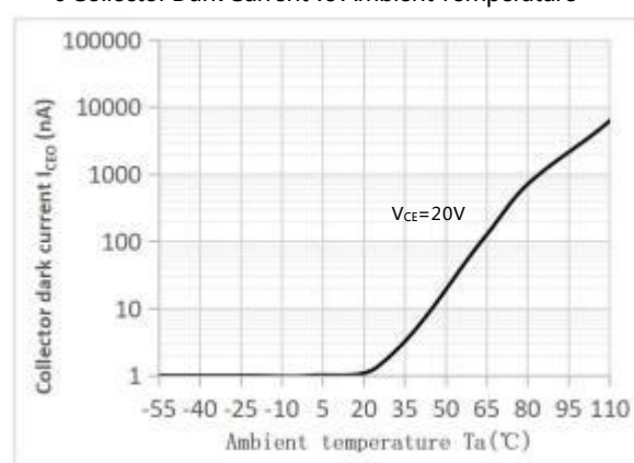
6 Collector Dark Current vs Ambient Temperature
