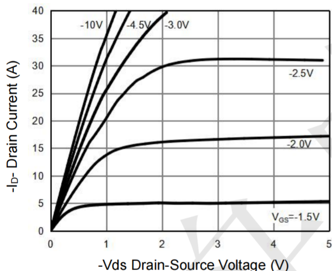
Figure 3 Output Characteristics
