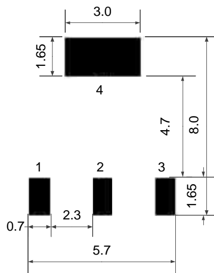
PCB Board
