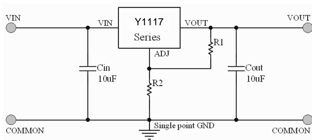
Application Circuit of Y1117-ADJ
