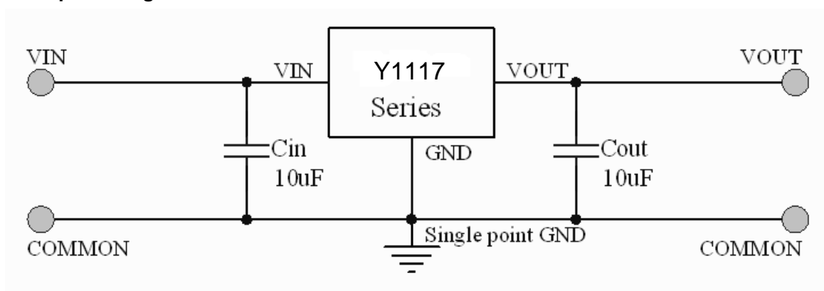
Application circuit of Y1117 fixed version
