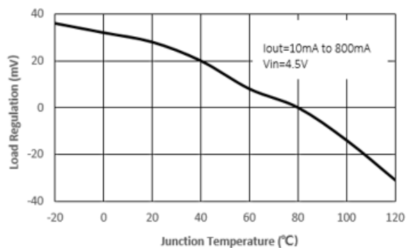
Load Regulation vs. Junction Temperature
