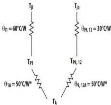
Figure. 41 ACPL-333J(AT) thermal model
