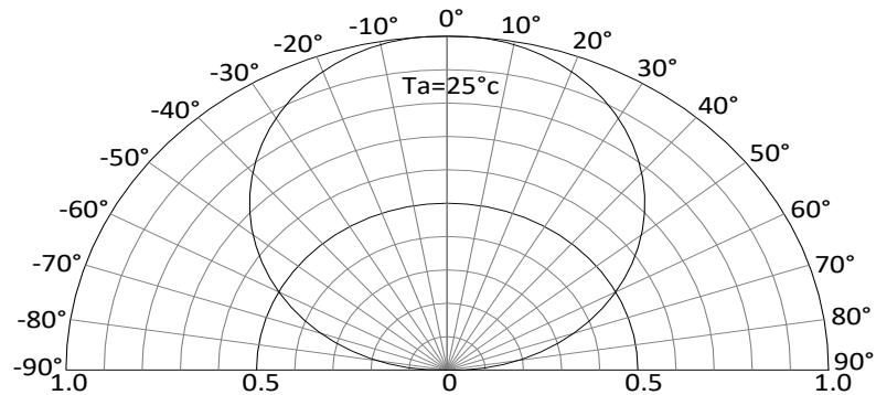
Radiation Pattern
