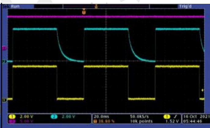
Fig4 Enable ON/OFF
