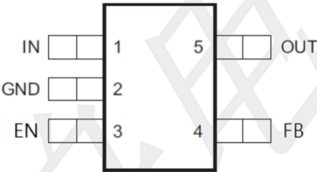
SOT23-5(TOP VIEW)
