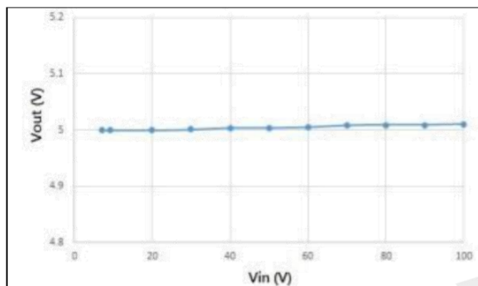
Fig1 V_{out} vs V_{in}
