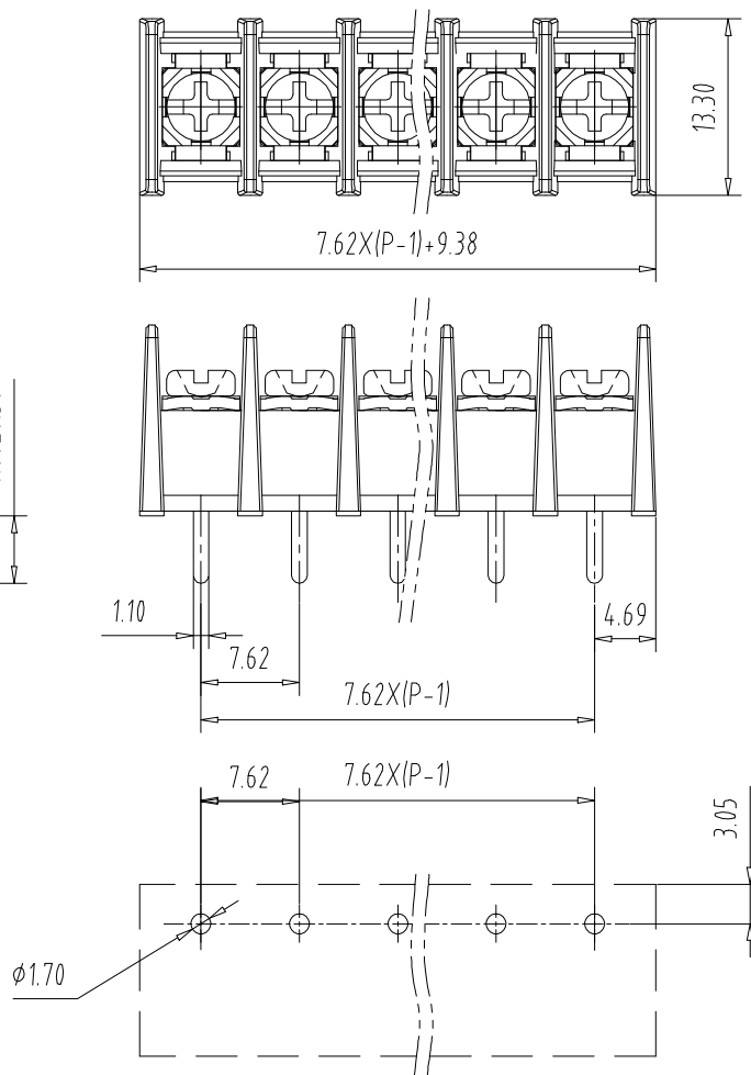
PCB Layout
