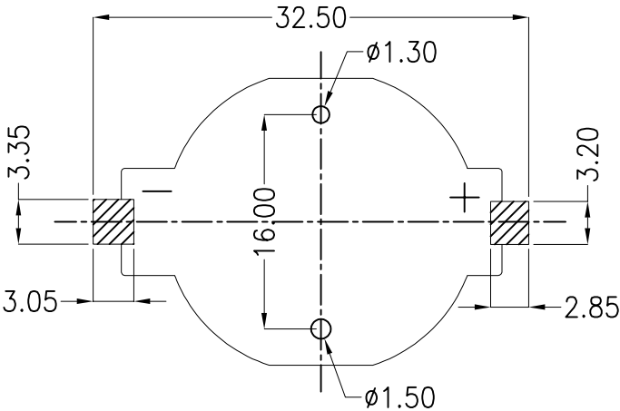
PCB Layout Diagram Top View
