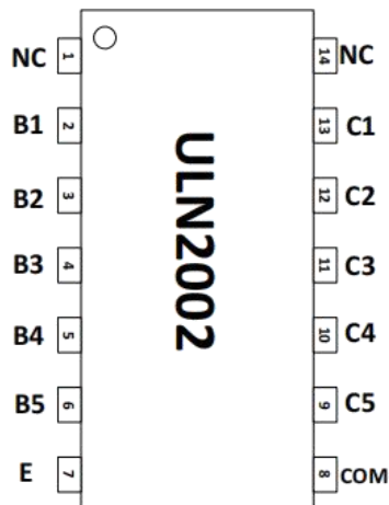
DIP-14/SOP-14/TSSOP-14
