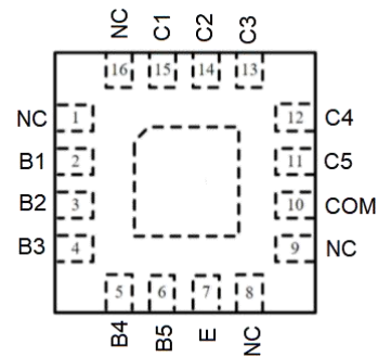
QFN-16 3*3
