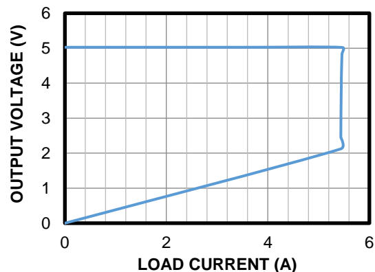
CC/CV Curve
