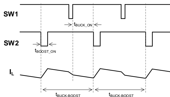
Figure 5: Buck-Boost Waveform
