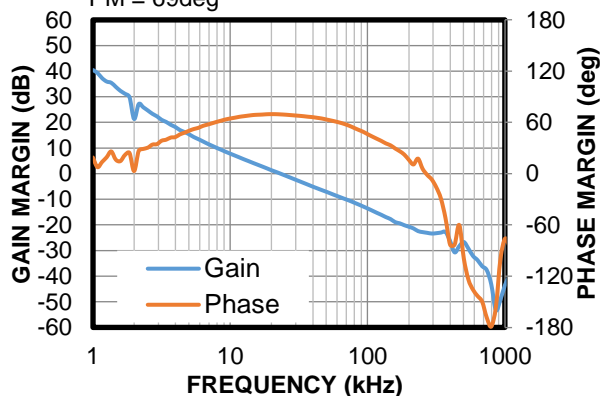
Bode Plot
