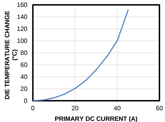
Figure 10: Self-Heating Performance with DC Input Current
