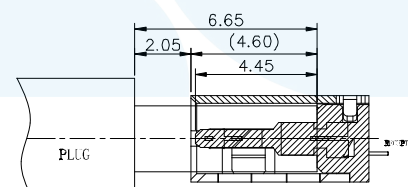
AFTER MATING SCALE 1:1
