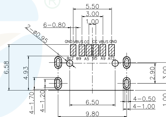
RECOMMENDED PCB LAYOUT(TOP VIEW) DEFAULT TOLERANCE+/-0.05
