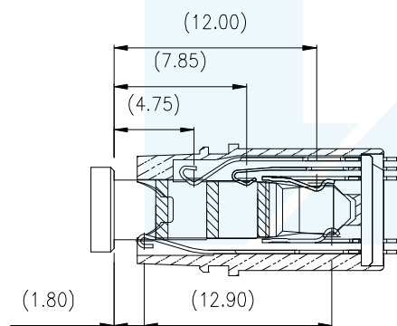
CROSS SECTION MATING REFERENCE DRAWING
