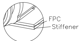
Detail A (scale 2:1)
