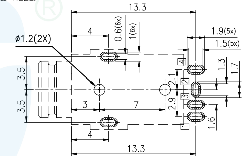
Recommended PCB Layout(T=1.2) Tolerance: ±0.05(TOP view)
