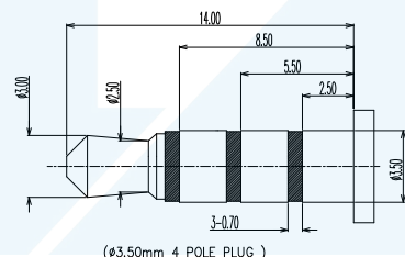
(ø3.50mm 4 POLE PLUG )
