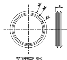
WATERPROOF RING
