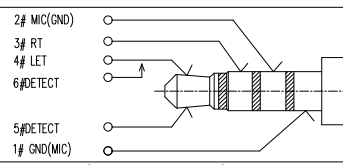
(ø1.50mm 4 POLE PLUG SCHEMATIC )
