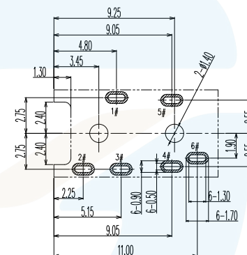
P.C.B LAYOUT T=1.00mm TOP VIEW
