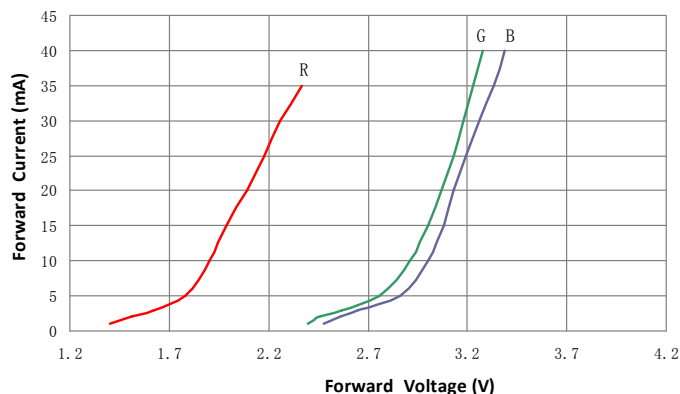
Forward Current VS. Forward Voltage ( T_a=25^\circ\text{C} )
