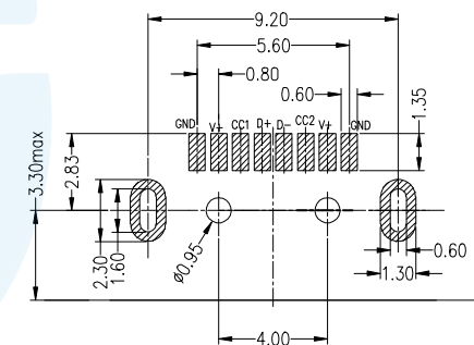
RECOMMEND PCB LAYOUT TOL=±0.05_(TOP VIEW)
