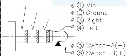
Circuit Diagram
