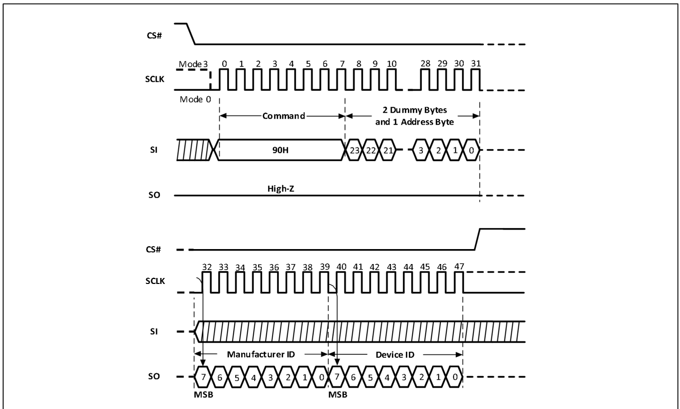
Figure-24. Read Electronic Manufacturer ID &amp; Device ID Sequence Diagram
