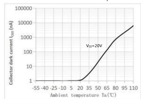
6 Collector Dark Current vs Ambient Temperature
