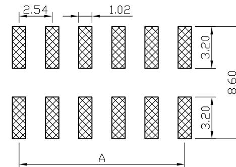
RECOMMEND P. C. B LAYOUT PCB TOLERANCE: \pm 0.05 (TOP VIEW)
