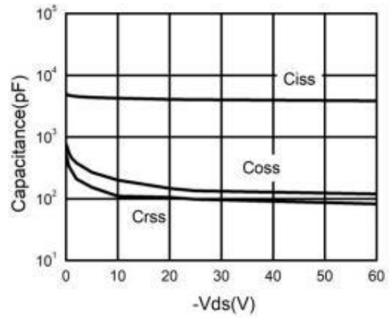
Figure 8. Capacitance
