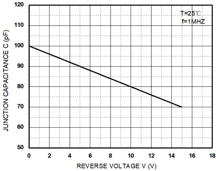
Capacitance Characteristics
