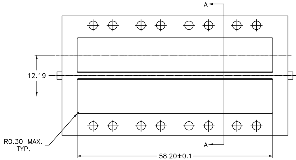
RECOMMENDED BEZEL DESIGN BELLY TO BELLY APPLICATIONS
