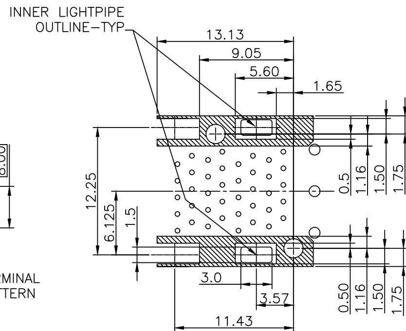
DETAIL-KEEPOUT ZONES
