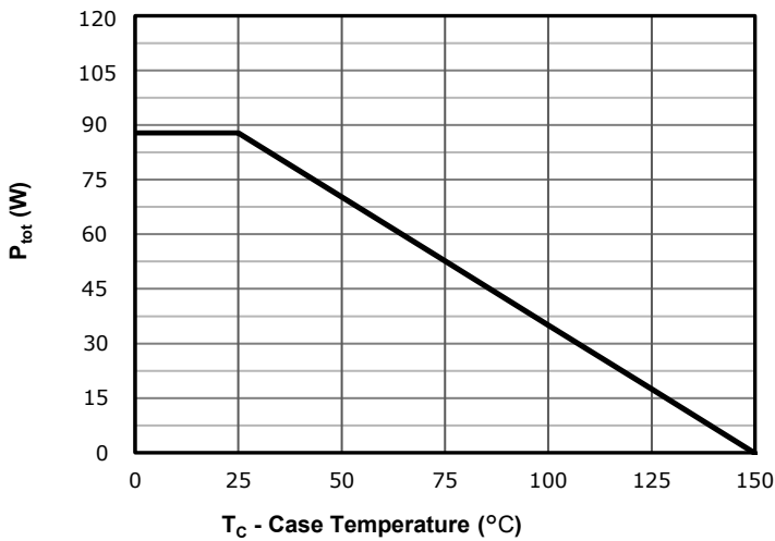
Fig 9: Power Dissipation
