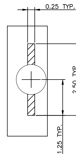
DETAIL "B" 10:1
