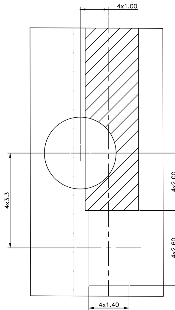
DETAIL "A" 10:1
