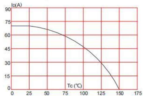
Figure 10: Maximum Continuous Drain Current vs. Case Temperature
