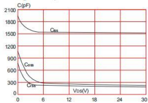
Figure 6: Capacitance Characteristics
