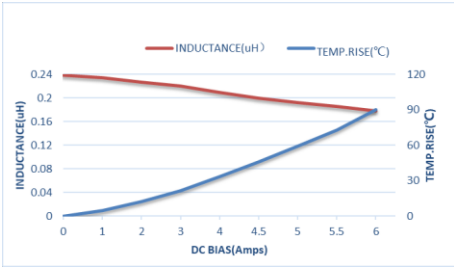
ZEMS160808-R22M
