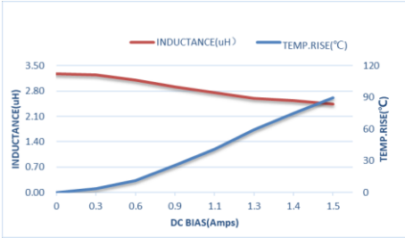
ZEMS160808-3R3M
