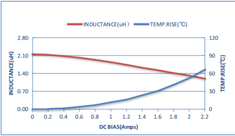
ZEMS160808-2R2M
