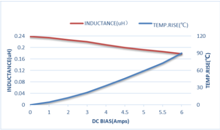
ZEMS160808-R24M
