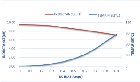
ZEMS160808-100M
