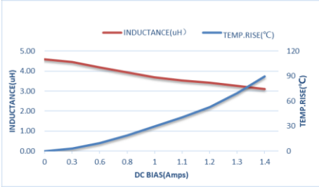
ZEMS160808-4R7M
