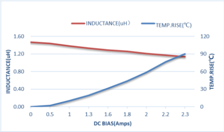
ZEMS160808-1R5M
