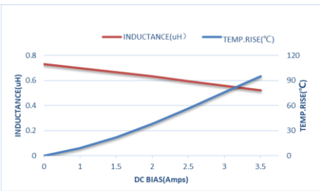
ZEMS160808-R68M
