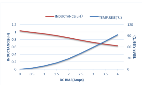
ZEMS160808-1R0M
