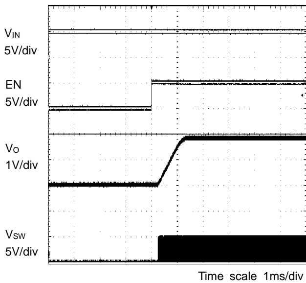
Figure 19. Start-up by EN V_{IN} = 5.0V, V_O = 1.8V
