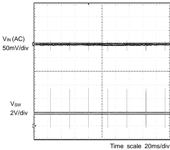
Figure 15. Input Voltage Ripple Wave
