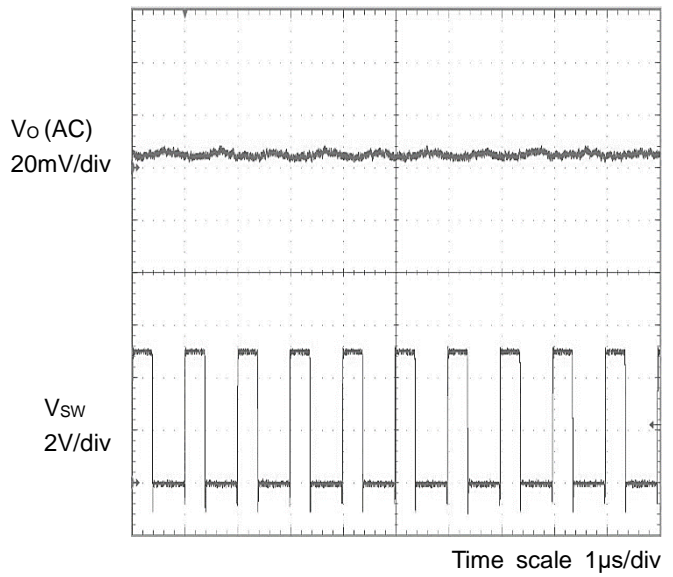
Figure 18. Output Voltage Ripple Wave V_{IN} = 5.0V, V_O = 1.8V, I_o=1A
