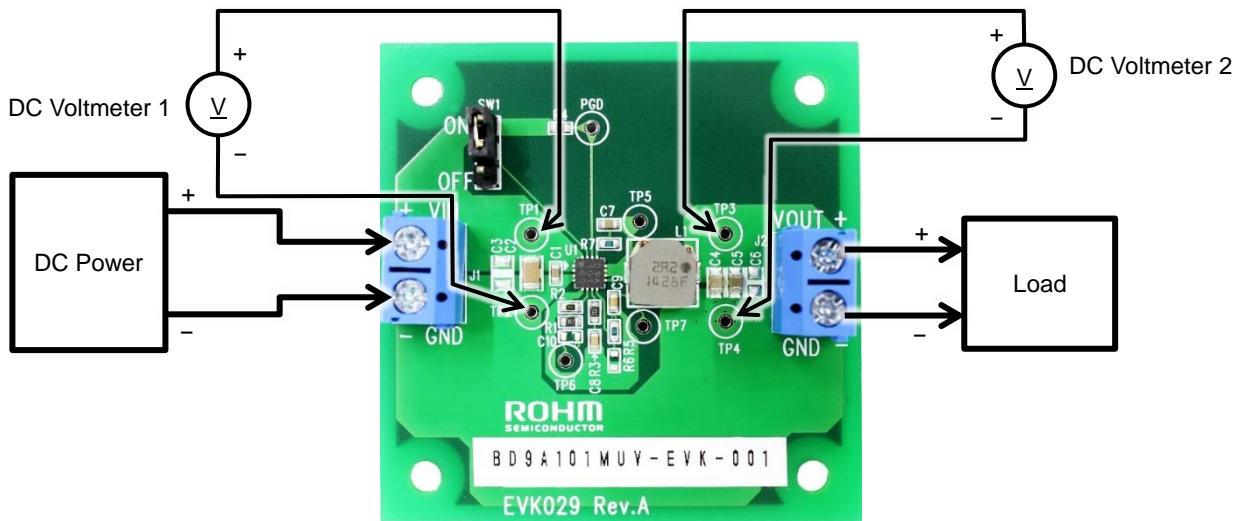
Figure 2. Connection Diagram
