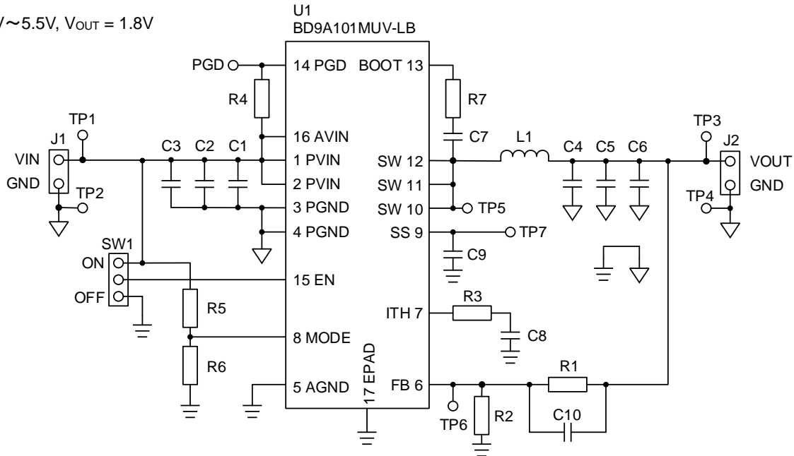
Figure 3. BD9A101MUV-EVK-001 Circuit Diagram
