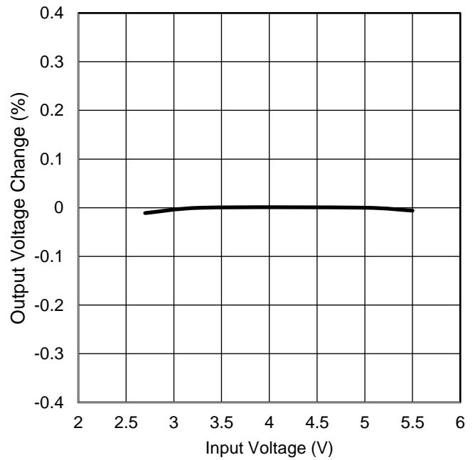
Figure 11. Line Regulation
