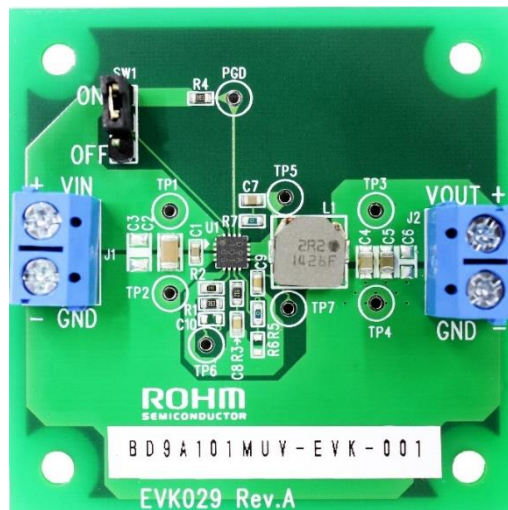
Figure 1. BD9A101MUV-EVK-001 Evaluation Board
