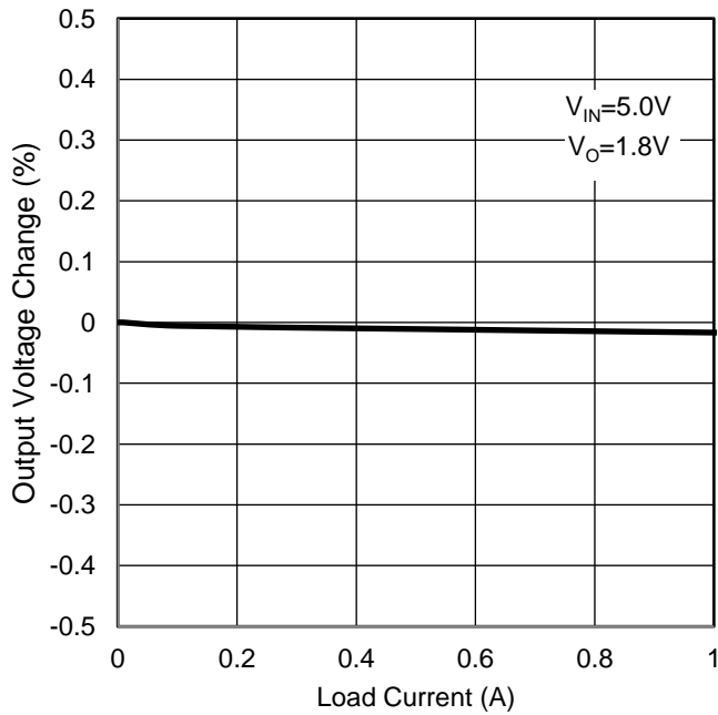
Figure 12. Load Regulation
