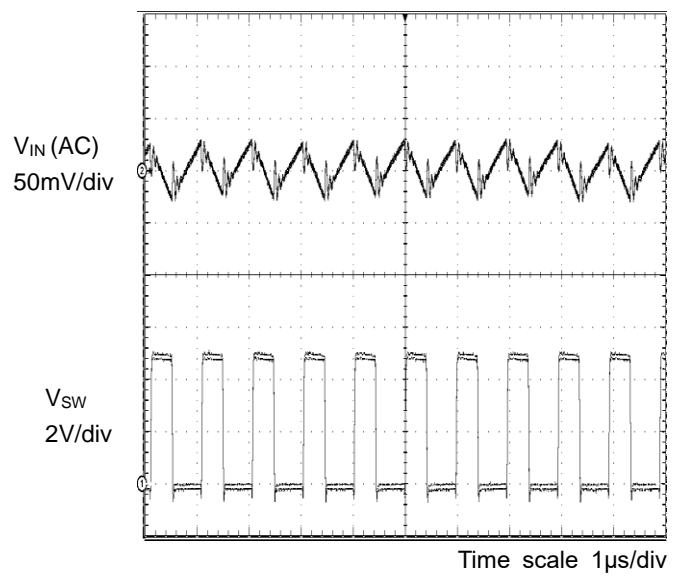
Figure 16. Input Voltage Ripple Wave
