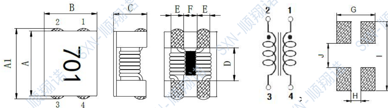
Land Pattern
