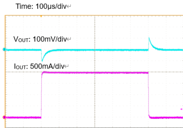
Figure 13. Load Transient Response (I OUT = 0 A ↔ 1 A)
