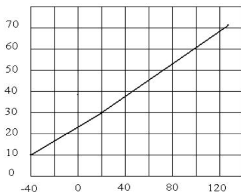
Off-State Cathode Current I_{Koff} (uA) vs. Junction Temperature T_J (°C) U_K=36V
