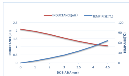
ZET-CORE-252008ST2R2MBCA
