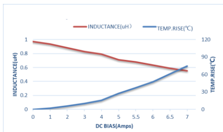
ZET-CORE-252008ST1R0MBCA
