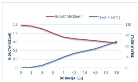
ZET-CORE-252008ST1R5MBCA
