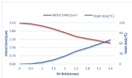
ZET-CORE-252008ST3R3MBCA
