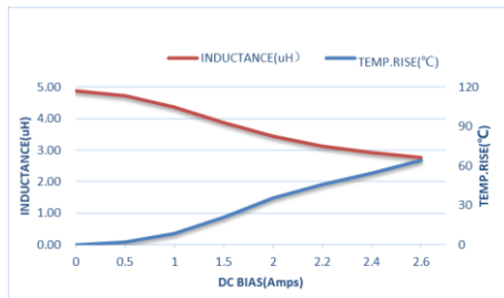
ZET-CORE-252008ST4R7MBCA
