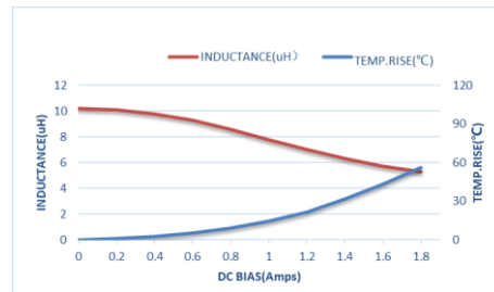
ZET-CORE-252008ST100MBCA
