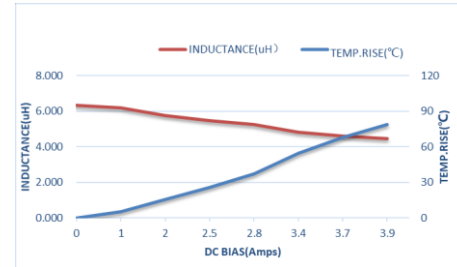
ZET-CORE-322520ST6R8MBCA
