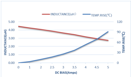
ZET-CORE-322520ST4R7MBCA
