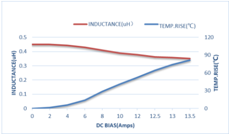
ZET-CORE-322520STR47MBCA
