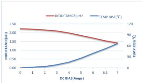
ZET-CORE-322520ST2R2MBCA
