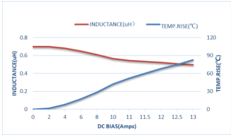
ZET-CORE-322520STR68MBCA
