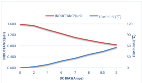
ZET-CORE-322520ST1R5MBCA
