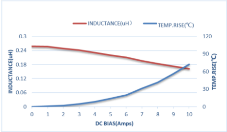
ZEMS201610-R22M
