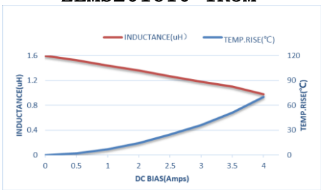
ZEMS201610-1R5M
