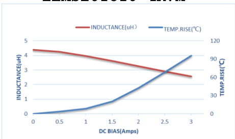
ZEMS201610-4R7M
