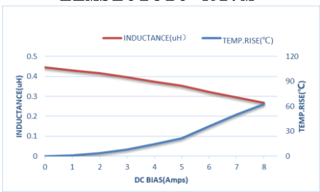
ZEMS201610-R47M
