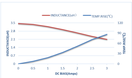
ZEMS201610-3R3M
