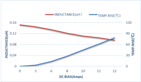
ZEMS201610-R15M
