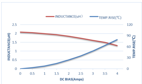
ZEMS201610-2R2M
