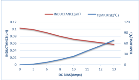
ZEMS201610-R10M
