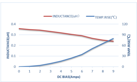
ZEMS201610-R33M
