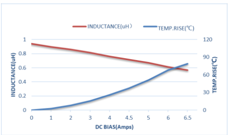
ZEMS201610-1R0M
