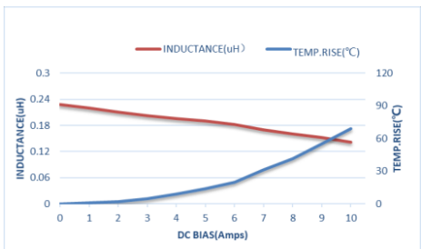
ZEMS201610-R24M
