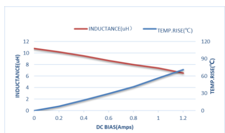
ZEMS201610-100M
