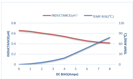
ZEMS201610-R68M
