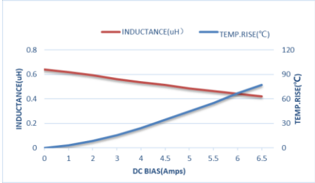
ZET-CORE-201210STR68MBCA
