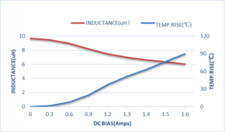
ZET-CORE-201210ST100MBCA
