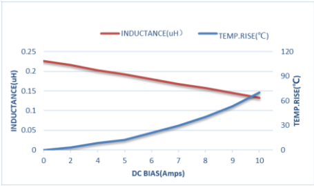
ZET-CORE-201210STR22MBCA
