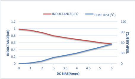
ZET-CORE-201210ST1R0MBCA
