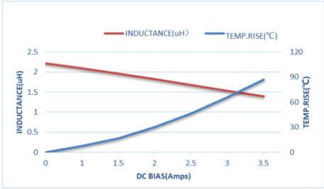
ZET-CORE-201210ST2R2MBCA
