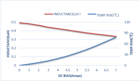
ZET-CORE-201210STR47MBCA
