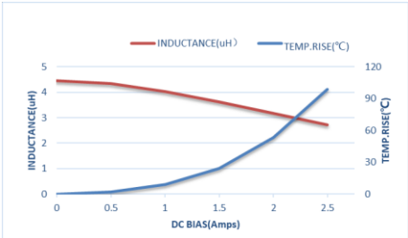
ZET-CORE-201210ST4R7MBCA
