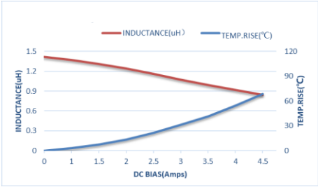
ZET-CORE-201210ST1R5MBCA
