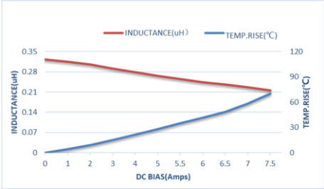
ZET-CORE-201210STR33MBCA
