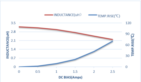
ZET-CORE-201210ST3R3MBCA
