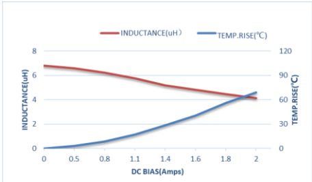
ZET-CORE-201210ST6R8MBCA
