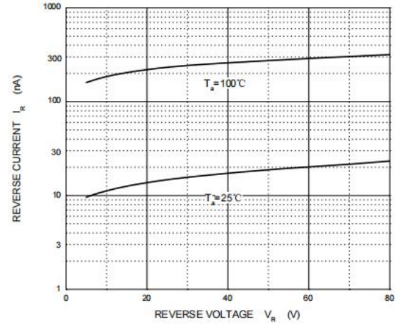
Figure 2: Leakage Current
