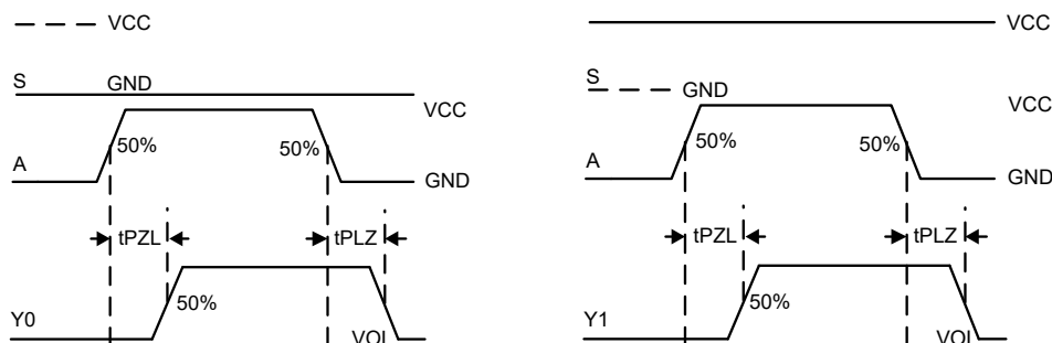
Figure 3/4 Switching Waveform
