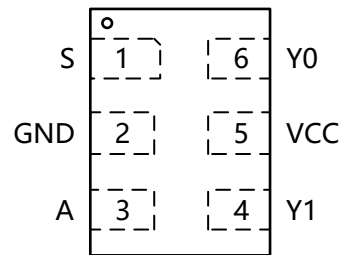
DFN6 (1*1.5)
