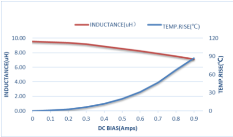
ZET-CORE-160808ST100MBCA
