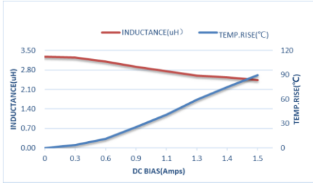
ZET-CORE-160808ST3R3MBCA
