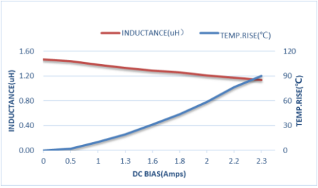
ZET-CORE-160808ST1R5MBCA
