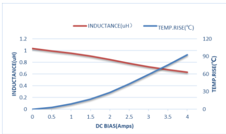
ZET-CORE-160808ST1R0MBCA
