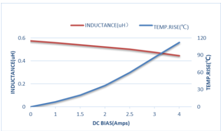
ZET-CORE-160808STR56MBCA
