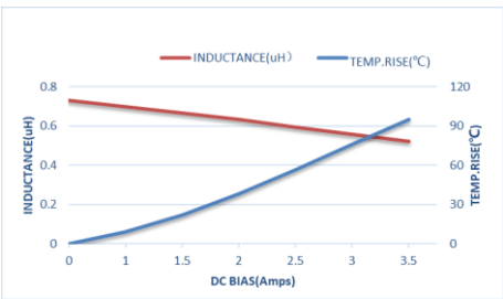
ZET-CORE-160808STR68MBCA
