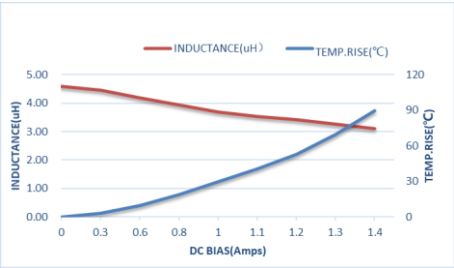
ZET-CORE-160808ST4R7MBCA
