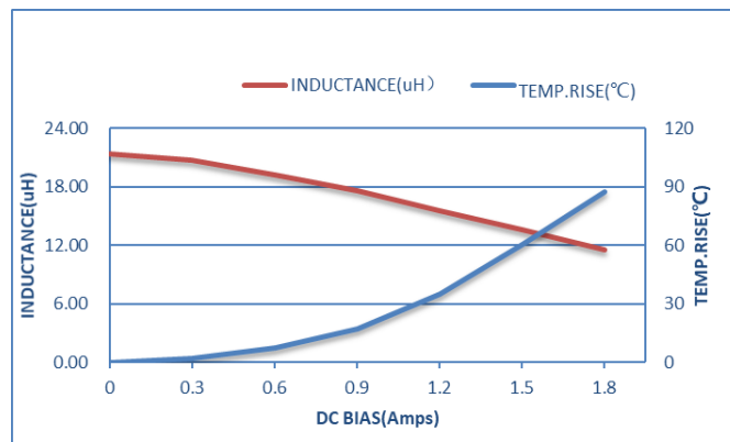
ZET-CORE-252012ST220MBCA
