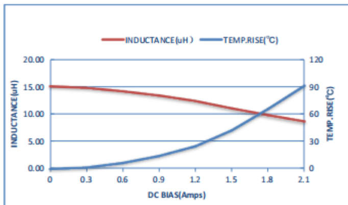
ZET-CORE-252012ST150MBCA
