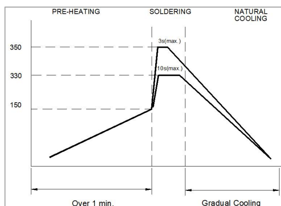
Figure 2. Hand Soldering
