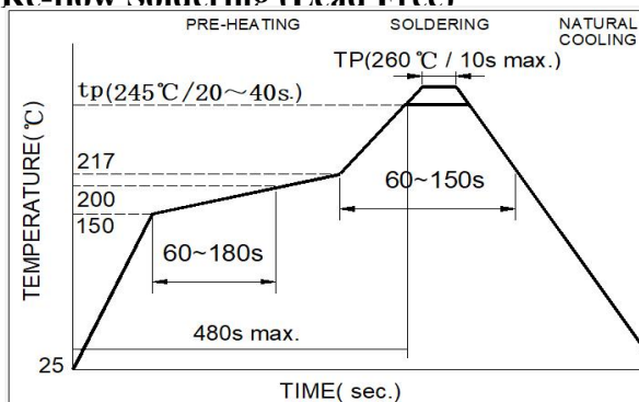
Figure 1. Re-flow Soldering (Lead Free)
