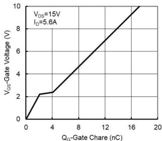
Figure 6: Gate-Charge Characteristics
