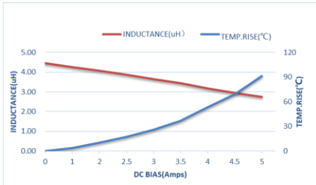
ZEMS322520-4R7M
