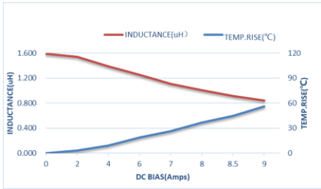
ZEMS322520-1R5M
