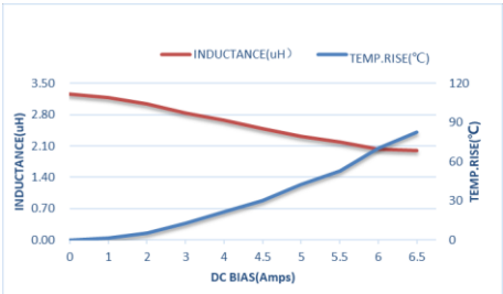
ZEMS322520-3R3M
