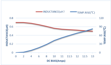
ZEMS322520-R68M
