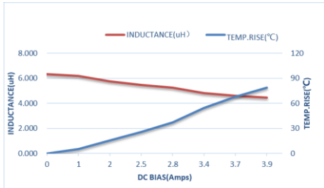
ZEMS322520-6R8M
