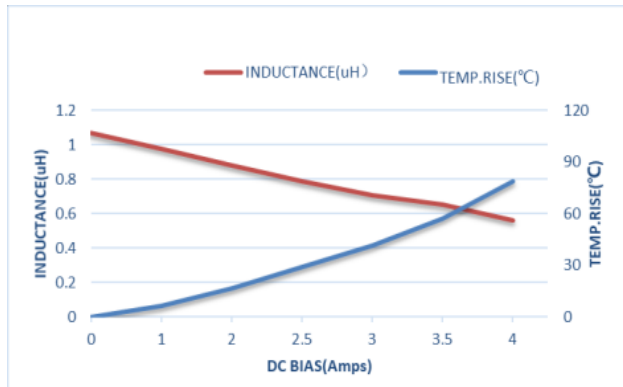
ZEMS201265-1R0M
