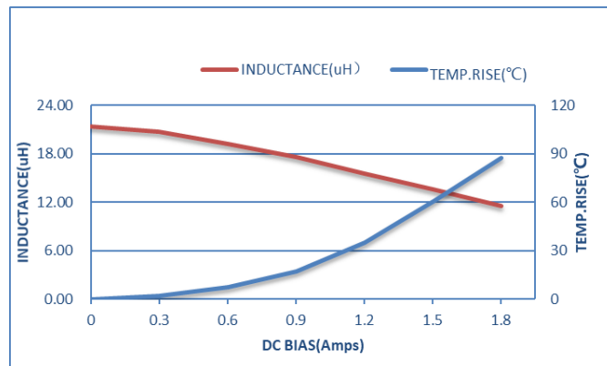
ZET-CORE-252012ST220MBCA
