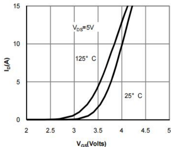
Figure 4: Transfer Characteristics
