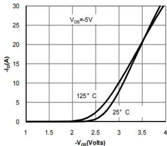
Figure 4: Transfer Characteristics
