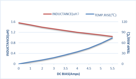
ZET-CORE-252012ST1R5MBCA
