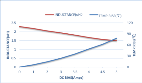
ZET-CORE-252012ST2R2MBCA
