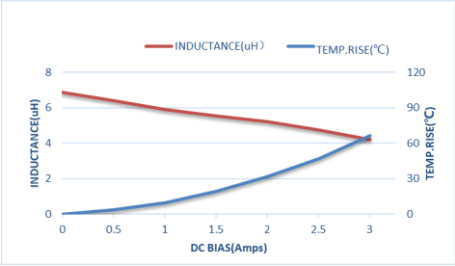
ZET-CORE-252012ST6R8MBCA
