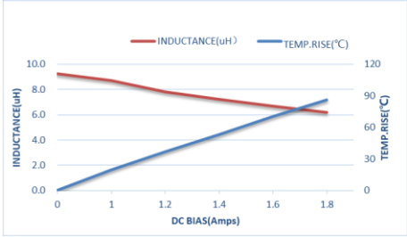
ZET-CORE-252012ST100MBCA
