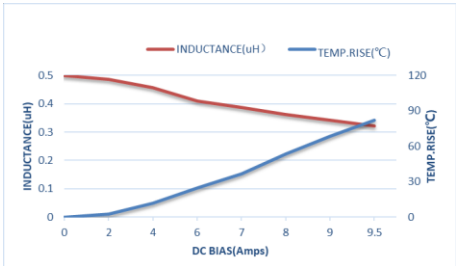
ZET-CORE-252012STR47MBCA
