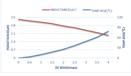
ZET-CORE-252012ST3R3MBCA
