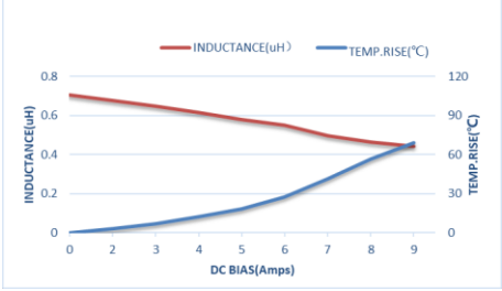
ZET-CORE-252012STR68MBCA
