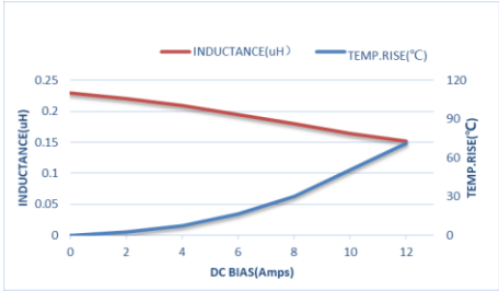
ZET-CORE-252012STR22MBCA
