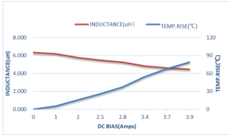
ZEP1M322520S-6R8M
